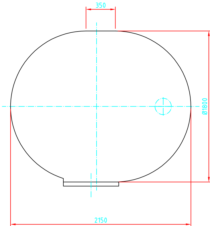
Forno \varnothing 135 TWISTER LEGNA SIDE
